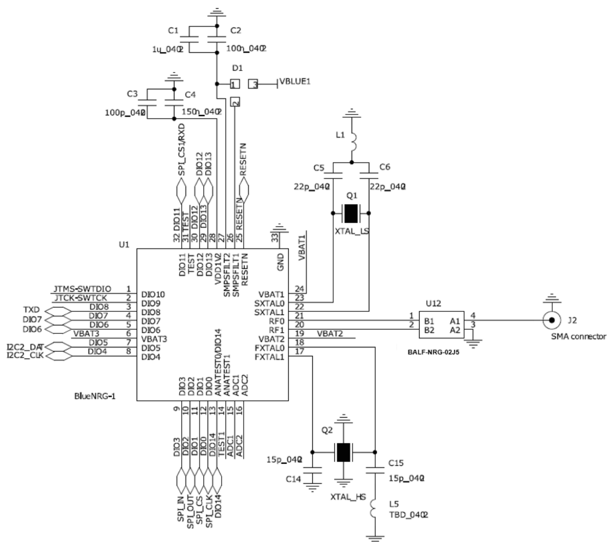
Figure 1. Application schematic
