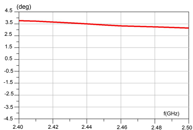
Figure 13. Phase imbalance ( T_{amb} = 25\text{ }^{\circ}\text{C} )
