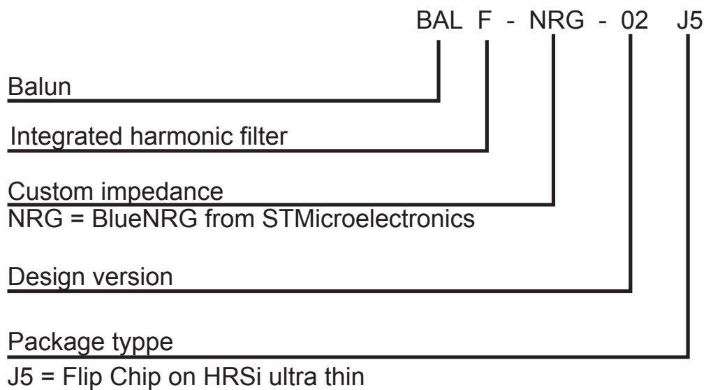
Figure 20. Ordering information scheme
