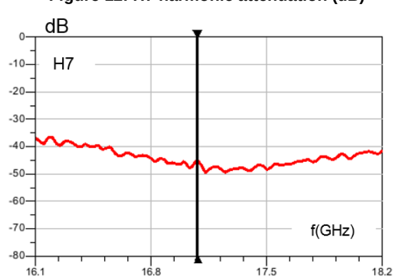
Figure 12: H7 harmonic attenuation (dB)
