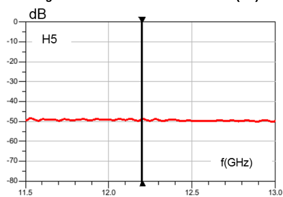
Figure 10: H5 harmonic attenuation (dB)
