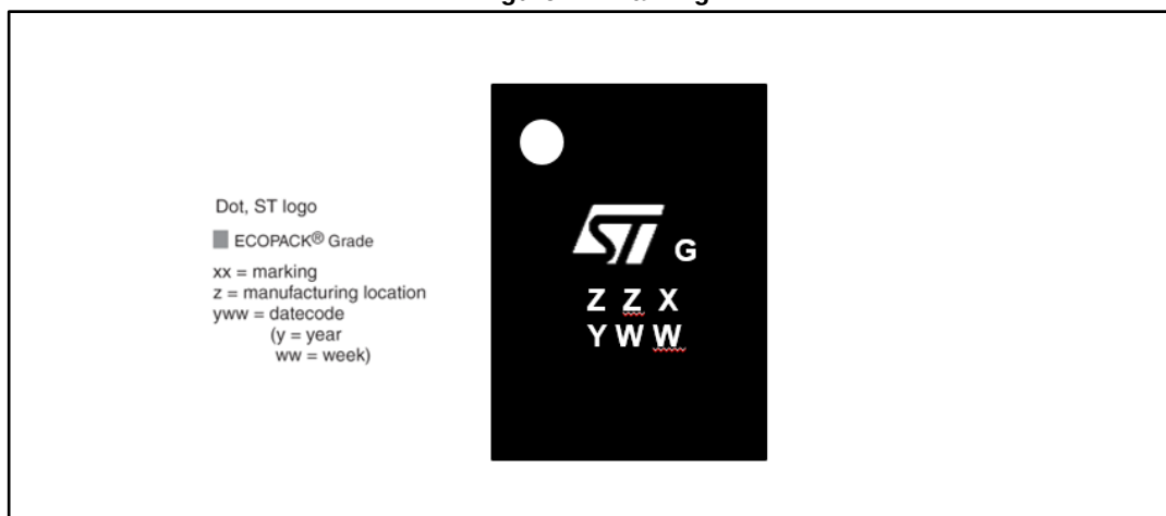
Figure 21: Marking
