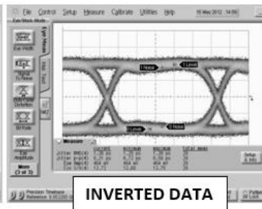
Fig. 1. Oscilloscope measurements of the BAL-0010 with a 10 Gb/s PRBS pattern. Bit pattern is measured with a 2^7-1 PRBS input demonstrating extremely good pulse fidelity for both inverted and non-inverted output. Eye diagrams are taken with a 2^{31}-1 PRBS input demonstrating minimal eye distortion/closure afforded by the extremely low frequency operation of the balun (<200 kHz).
