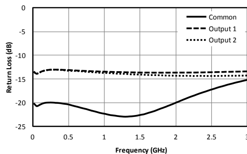
Fig. 11. Return loss for common port and output ports.
