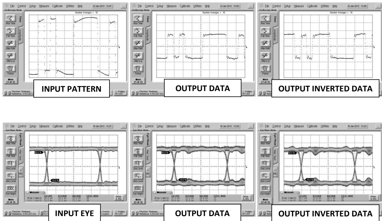
Fig. 1. Oscilloscope measurements of the BAL-0003SMG with a 3 Gb/s PRBS pattern. Bit pattern is measured with a 2^7-1 PRBS input demonstrating extremely good pulse fidelity for both inverted and non-inverted output. Eye diagrams are taken with a 2^{31}-1 PRBS input demonstrating minimal eye distortion/closure afforded by the extremely low frequency operation of the balun (<500 kHz).
