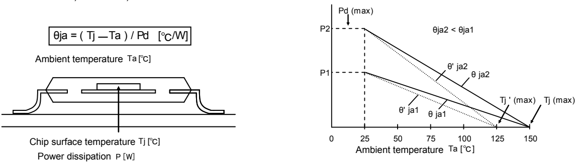
(a) Thermal resistance (b) Derating curve Fig.91 Thermal resistance and derating curve
