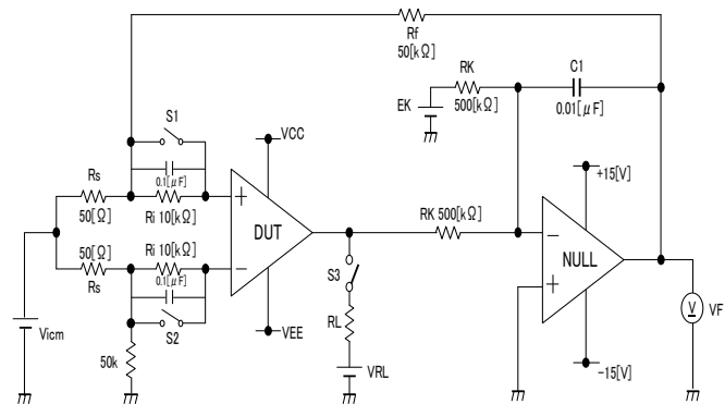
Fig.88 Measurement circuit1 (one channel only)
