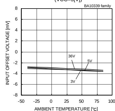
Fig.52 Input Offset Voltage - Ambient Temperature
