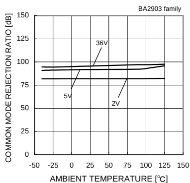
Fig.80 Common Mode Rejection Ratio - Ambient Temperature
