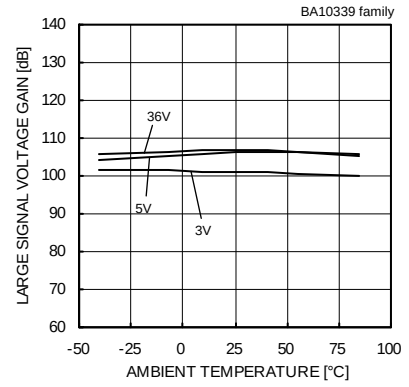
Fig.58 Large Signal Voltage Gain - Ambient Temperature
