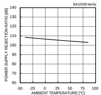
Fig.61 Power Supply Rejection Ratio - Ambient Temperature
