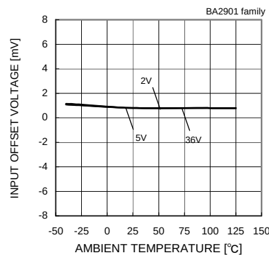
Fig.95 Input Offset Voltage - Ambient Temperature
