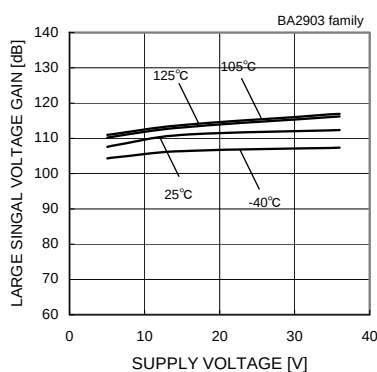
Fig.77 Large Signal Voltage Gain - Supply Voltage
