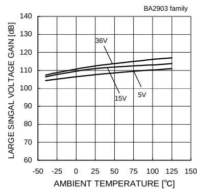
Fig.78 Large Signal Voltage Gain - Ambient Temperature
