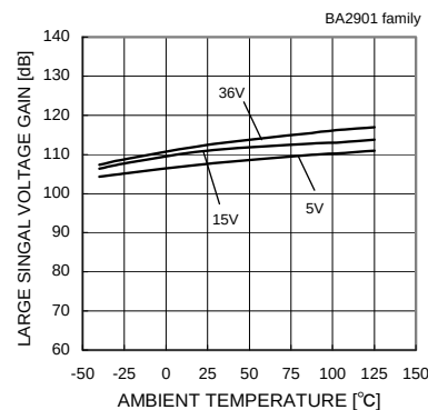
Fig.101 Large Signal Voltage Gain - Ambient Temperature
