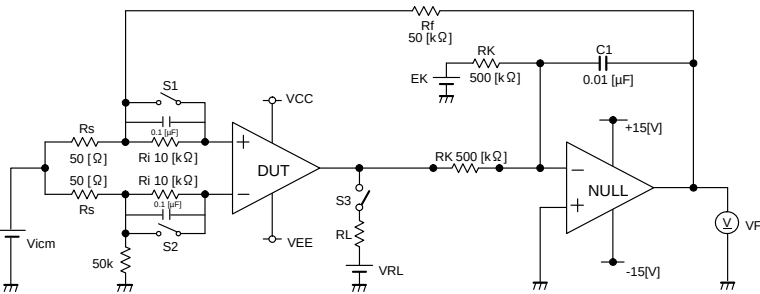
Fig.111 Test circuit1 (one channel only)
