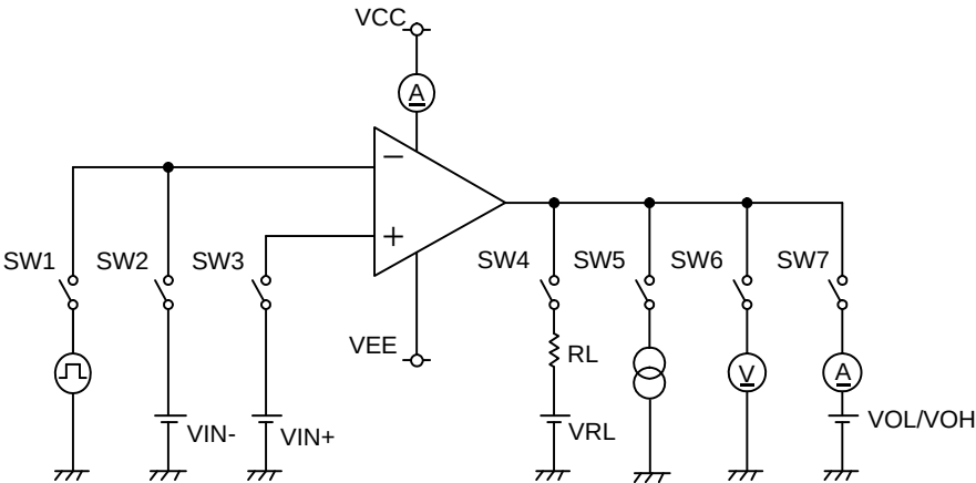
Fig.112 Test Circuit 2 (one channel only)
