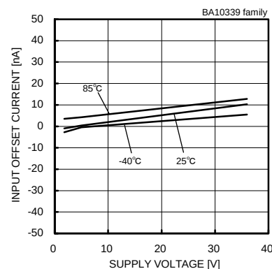
Fig.55 Input Offset Current - Supply Voltage
