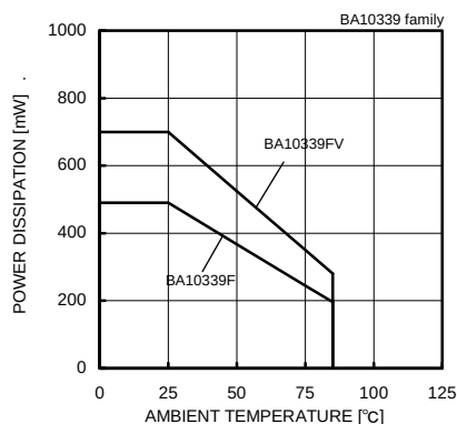
Fig.44 Derating Curve
