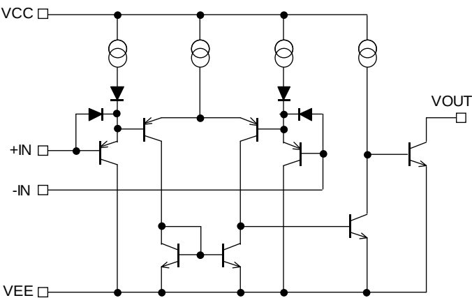
Fig.110 Schematic Diagram (one channel only)
