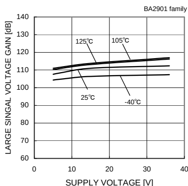
Fig.100 Large Signal Voltage Gain - Supply Voltage
