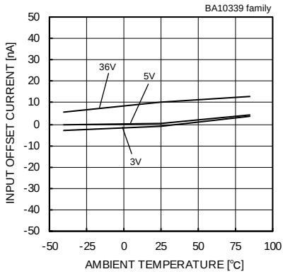
Fig.56 Input Offset Current - Ambient Temperature
