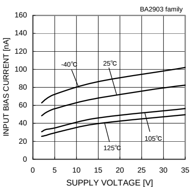
Fig.73 Input Bias Current - Supply Voltage
