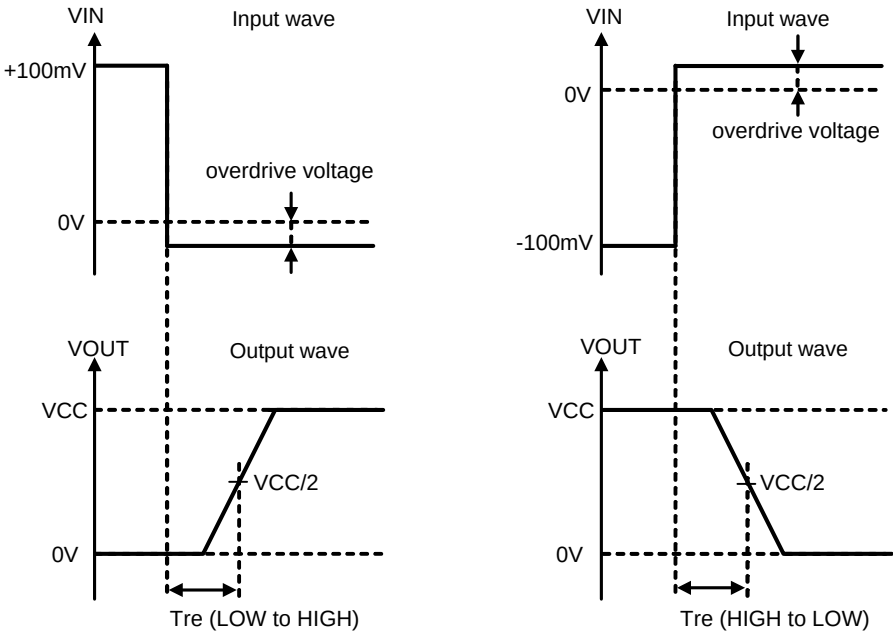
Fig.113 Response Time
