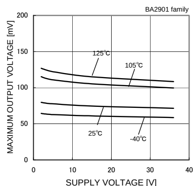
Fig.90 Output Saturation Voltage - Supply Voltage (IOL=4[mA])
