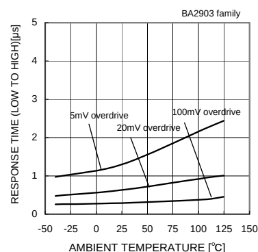
Fig.84 Response Time (Low to High) - Ambient Temperature (VCC=5[V],VRL=5[V],RL=5.1[kΩ])
