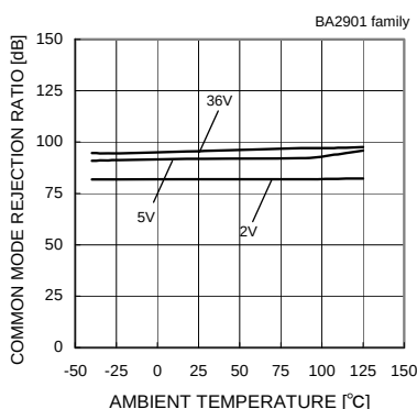
Fig.103 Common Mode Rejection Ratio - Ambient Temperature
