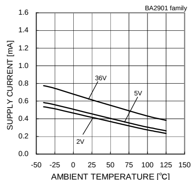
Fig.89 Supply Current - Ambient Temperature
