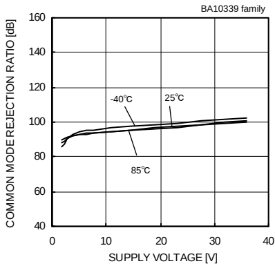
Fig.59 Common Mode Rejection Ratio - Supply Voltage
