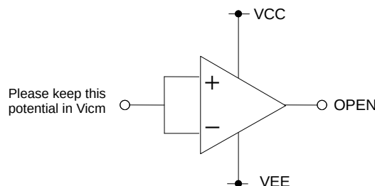
Fig.116 Disable circuit example
