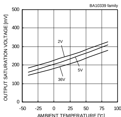
Fig.48 Output Saturation Voltage - Ambient Temperature (IOL=4[mA])
