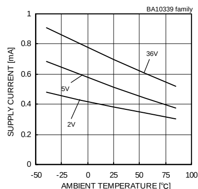
Fig.46 Supply Current - Ambient Temperature
