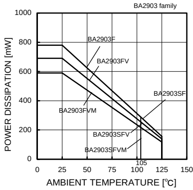
Fig.64 Derating Curve
