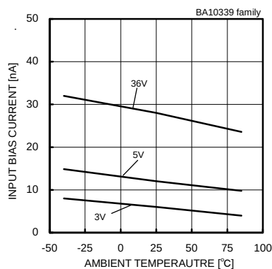
Fig.54 Input Bias Current - Ambient Temperature
