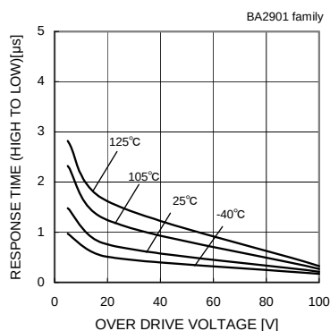
Fig.108 Response Time (High to Low) - Over Drive Voltage (VCC=5[V],VRL=5[V],RL=5.1[kΩ])
