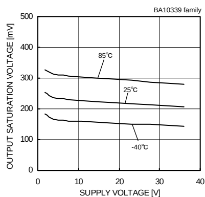
Fig.47 Output Saturation Voltage - Supply Voltage (IOL=4[mA])
