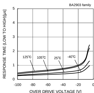
Fig.83 Response Time (Low to High) - Over Drive Voltage (VCC=5[V],VRL=5[V],RL=5.1[kΩ])
