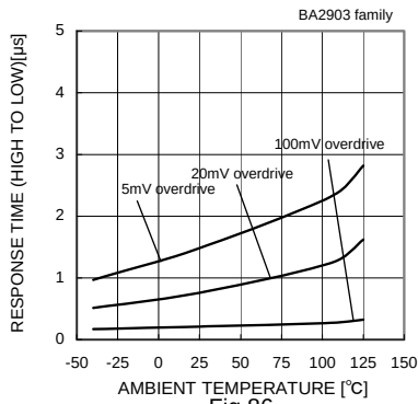
Fig.86 Response Time (High to Low) - Ambient Temperature (VCC=5[V],VRL=5[V],RL=5.1[kΩ])
