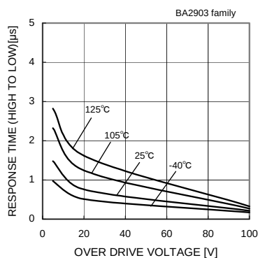
Fig.85 Response Time (High to Low) - Over Drive Voltage (VCC=5[V],VRL=5[V],RL=5.1[kΩ])
