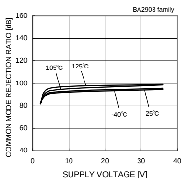
Fig.79 Common Mode Rejection Ratio - Supply Voltage
