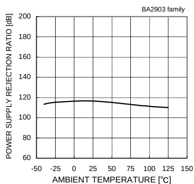
Fig.82 Power Supply Rejection Ratio - Ambient Temperature
