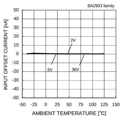
Fig.76 Input Offset Current - Ambient Temperature
