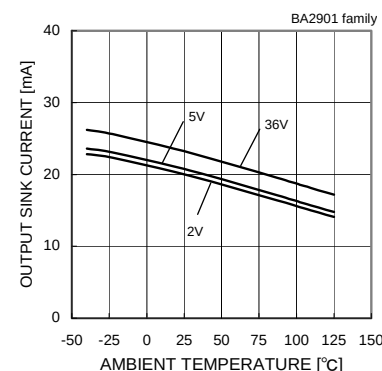
Fig.93 Output Sink Current - Ambient Temperature (VOUT=1.5[V])
