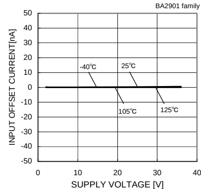
Fig.98 Input Offset Current - Supply Voltage
