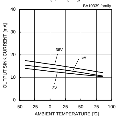
Fig.50 Output Sink Current - Ambient Temperature (VOUT=1.5[V])
