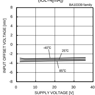
Fig.51 Input Offset Voltage - Supply Voltage
