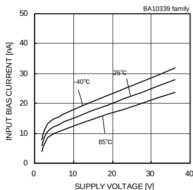
Fig.53 Input Bias Current - Supply Voltage
