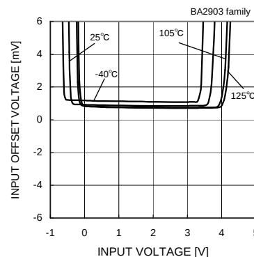
Fig.81 Input Offset Voltage - Input Voltage (VCC=5V)
