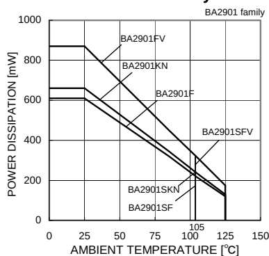
Fig.87 Derating Curve
