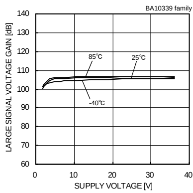
Fig.57 Large Signal Voltage Gain - Supply Voltage
