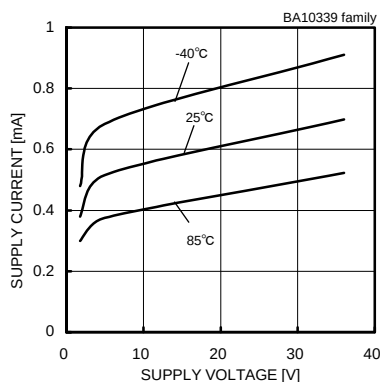
Fig.45 Supply Current - Supply Voltage
