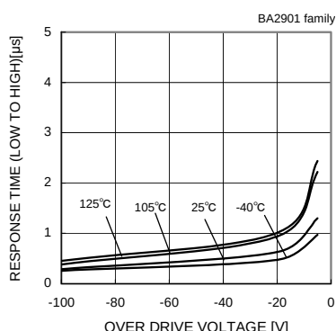
Fig.106 Response Time (Low to High) - Over Drive Voltage (VCC=5[V],VRL=5[V],RL=5.1[kΩ])
