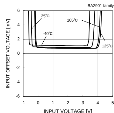
Fig.104 Input Offset Voltage - Input Voltage (VCC=5V)
