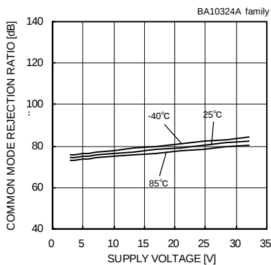
Common Mode Rejection Ratio - Supply Voltage
