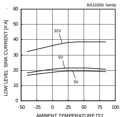
Low Level Sink Current - Ambient Temperature ( V_{OUT}=0.2[V] )
