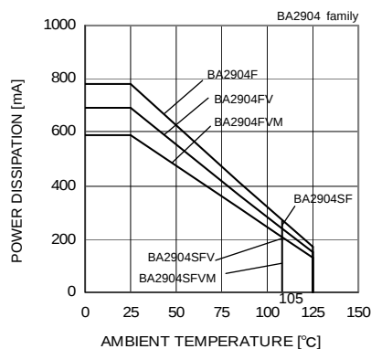
Fig. 49 Derating Curve
