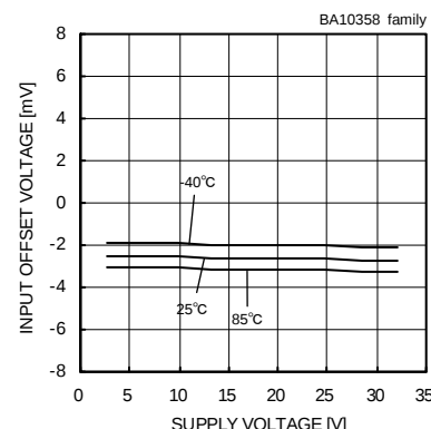
Input Offset Voltage - Supply Voltage ( V_{icm}=0[V] , V_{OUT}=1.4[V] )
