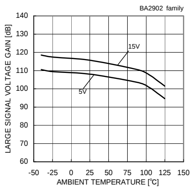
Large Signal Voltage Gain - Ambient Temperature ( R_L=2[k\Omega] )
