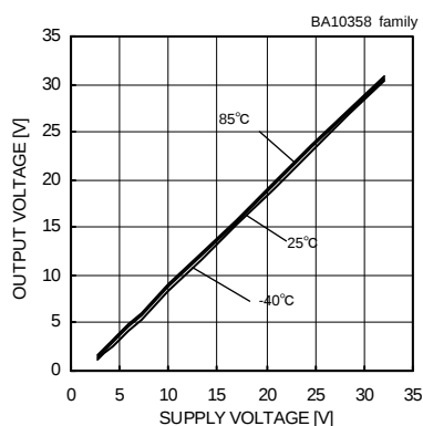
Maximum Output Voltage - Supply Voltage ( R_L=10[k\Omega] )
