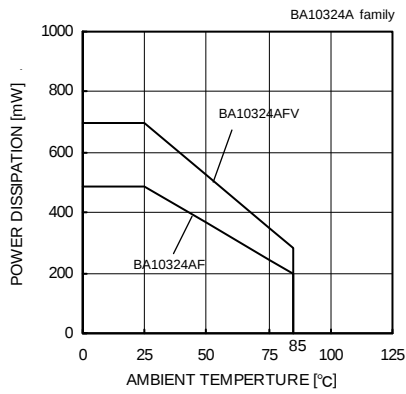
Fig. 25 Derating Curve
