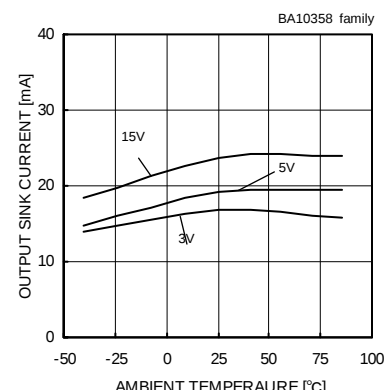
Output Sink Current - Ambient Temperature ( V_{OUT}=V_{CC} )
