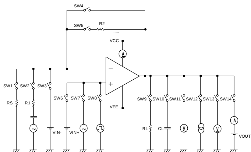
Fig.122 Test Circuit 2 (each Op-Amp)
