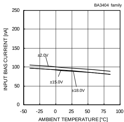
Fig. 106 Input Bias Current - Ambient Temperature (Vicm=0[V], VOUT=0[V])
