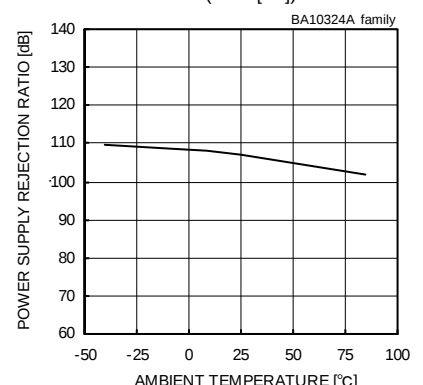
Power Supply Rejection Ratio - Ambient Temperature
