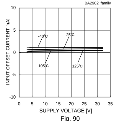
Input Offset Current - Supply Voltage ( V_{icm}=0[V] , V_{OUT}=1.4[V] )
