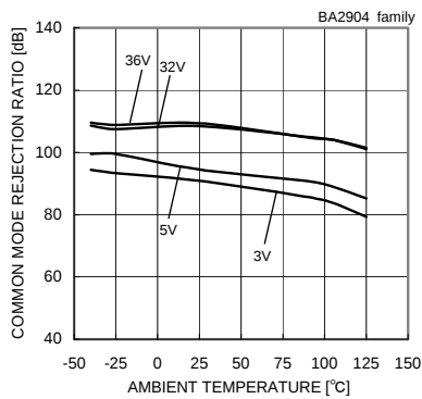
Fig. 71 Common Mode Rejection Ratio - Ambient Temperature
