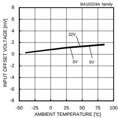
Input Offset Voltage - Ambient Temperature ( V_{icm}=0[V] , V_{OUT}=1.4[V] )
