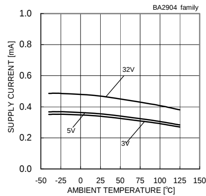
Fig. 51 Supply Current - Ambient Temperature
