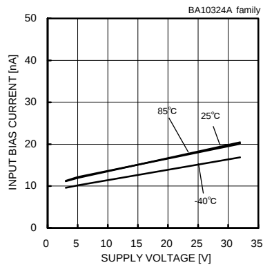
Input Bias Current - Supply Voltage ( V_{icm}=0[V] , V_{OUT}=1.4[V] )
