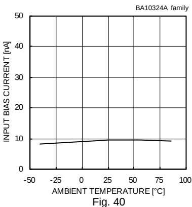
Input Bias Current - Ambient Temperature ( V_{CC}=30[V] , V_{icm}=28[V] , V_{OUT}=1.4[V] )
