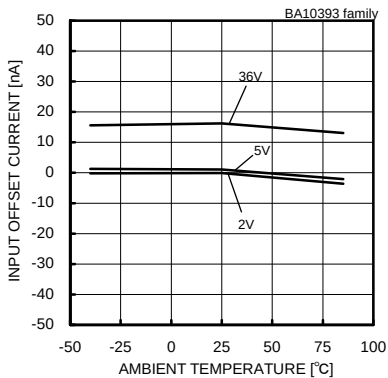
Fig. 13 Input Offset Current – Ambient Temperature
