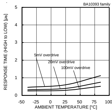
Fig. 20 Response Time (High to Low) – Ambient Temperature (VCC=5[V],VRL=5[V])
