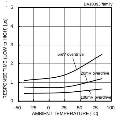
Fig. 19 Response Time (Low to High) – Ambient Temperature (VCC=5[V],VRL=5[V],RL=5.1[kΩ])
