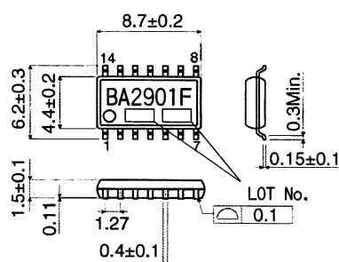
BA2901F(SOP14) (Unit:[mm])
