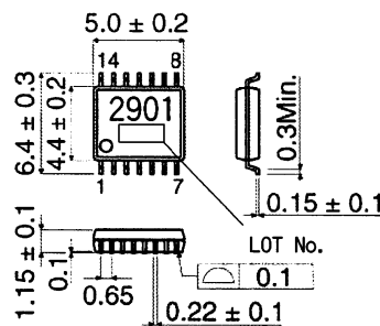
BA2901FV(SSOP-B14) (Unit:[mm])
