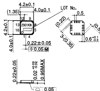
BA2901KN(VOFN16) (Unit:[mm])
