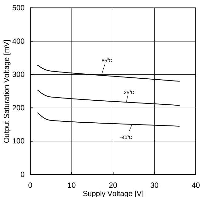
Figure 48. Output Saturation Voltage vs Supply Voltage (I OL =4mA)
