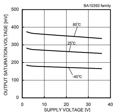
Fig.27 Output Saturation Voltage - Supply Voltage (IOL=4[mA])
