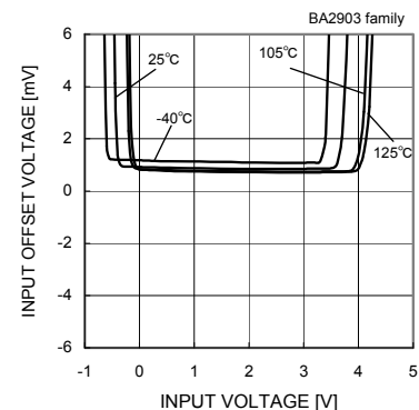
Fig.81 Input Offset Voltage - Input Voltage (VCC=5V)
