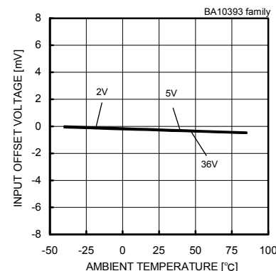
Fig.32 Input Offset Voltage - Ambient Temperature
