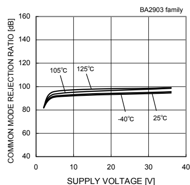
Fig.79 Common Mode Rejection Ratio - Supply Voltage
