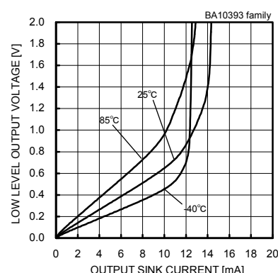
Fig.29 Low Level Output Voltage - Output Sink Current (VCC=5[V])
