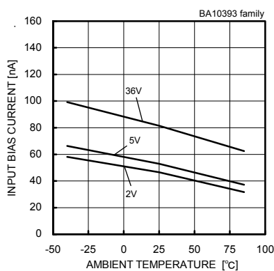
Fig.34 Input Bias Current - Ambient Temperature
