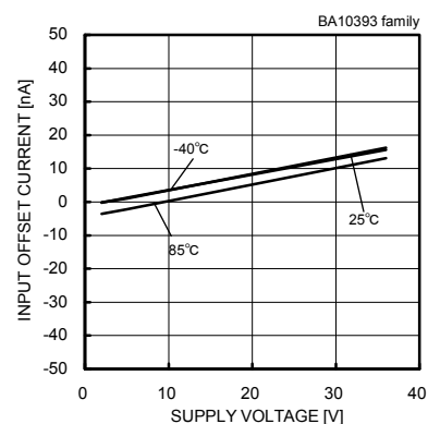
Fig.35 Input Offset Current - Supply Voltage
