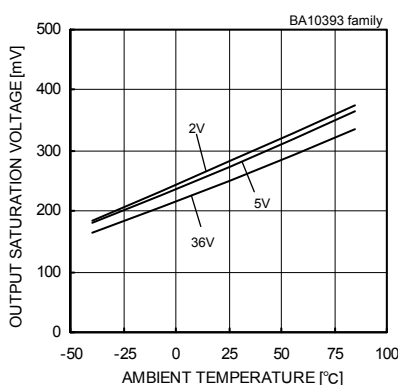
Fig.28 Output Saturation Voltage - Ambient Temperature (IOL=4[mA])
