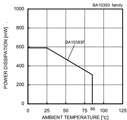
Fig.24 Derating Curve
