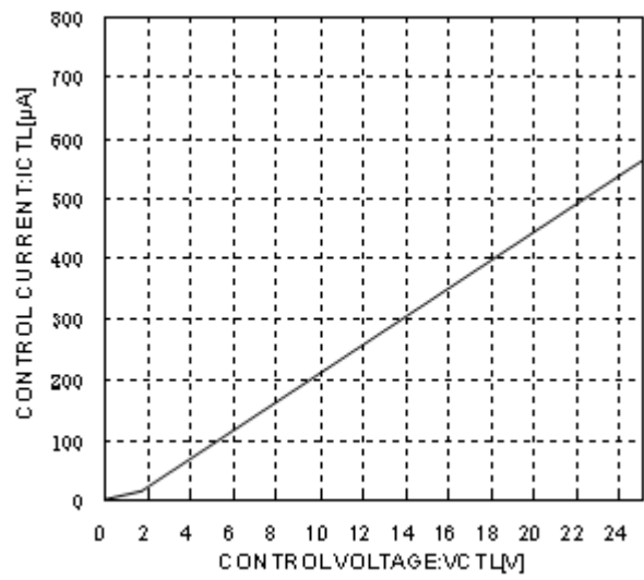
Fig.21 CTL Voltage vs. CTL Current
