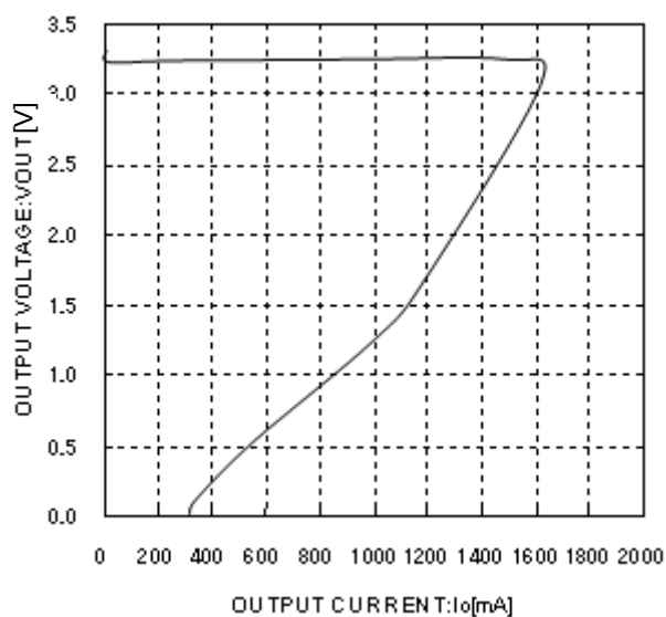
Fig.4 Load Stability
