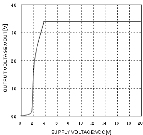
Fig.3 Input Stability ( I_o=500mA )
