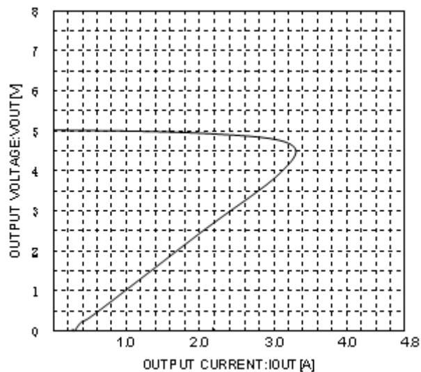
Fig.16 Load Stability
