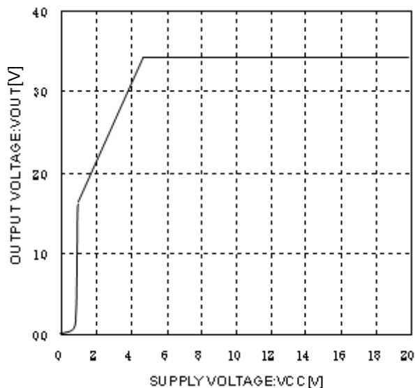
Fig.2 Input Stability
