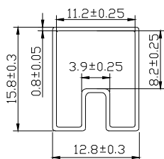
TUBE MECHANICAL DIMENSION
