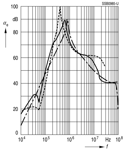
B84143-A120-R ... B84143-A180-R
