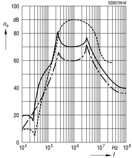
B84143-A25-R
