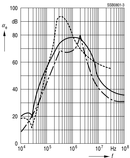
B84143-A25-R
