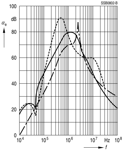
B84143-A80-R
