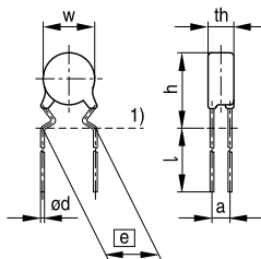
1) Seating plane to IEC 60717 VAR04111-F-E
