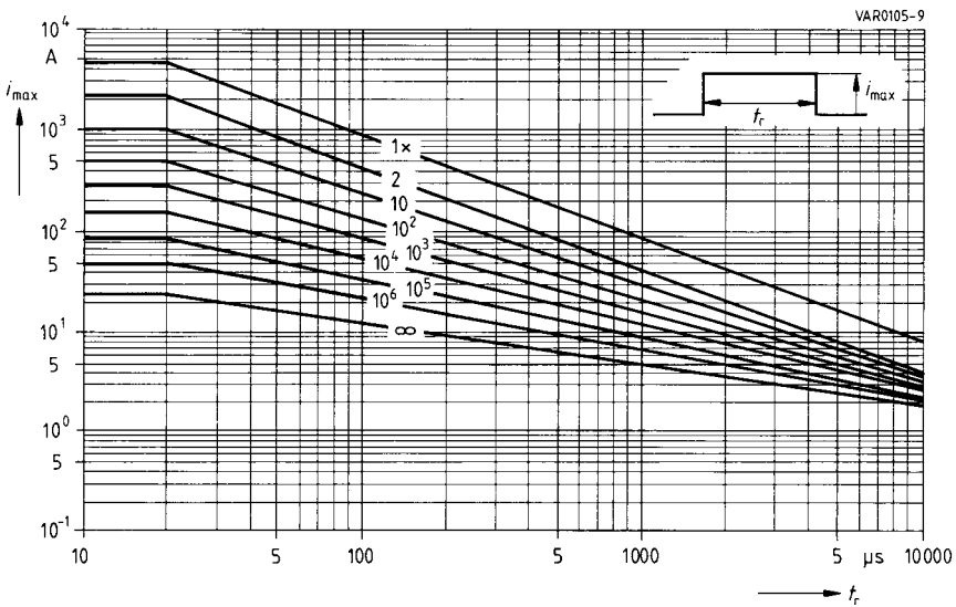
SIOV-S14K385 ... K1000
