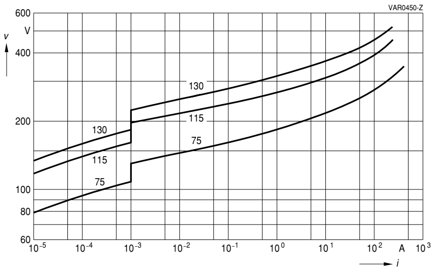
SIOV-CT/CN1812K75G2 ... K130G2
