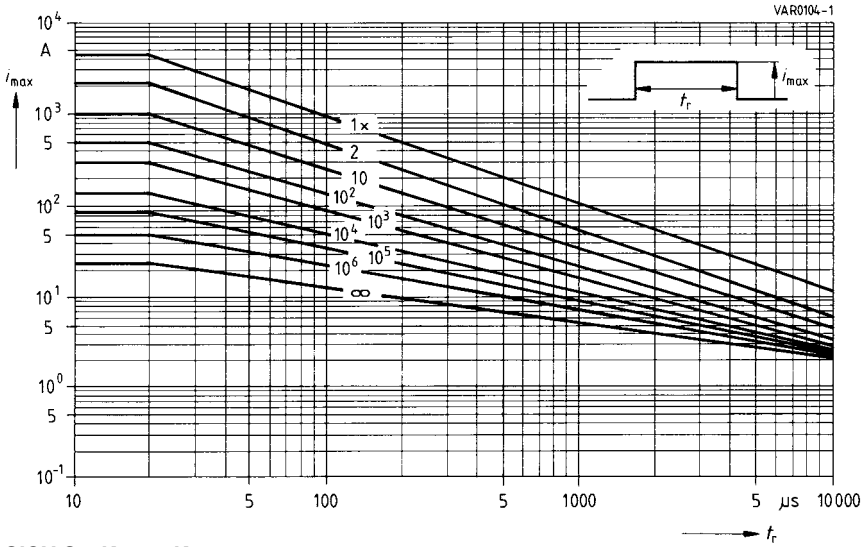
SIOV-S14K50 ... K320
