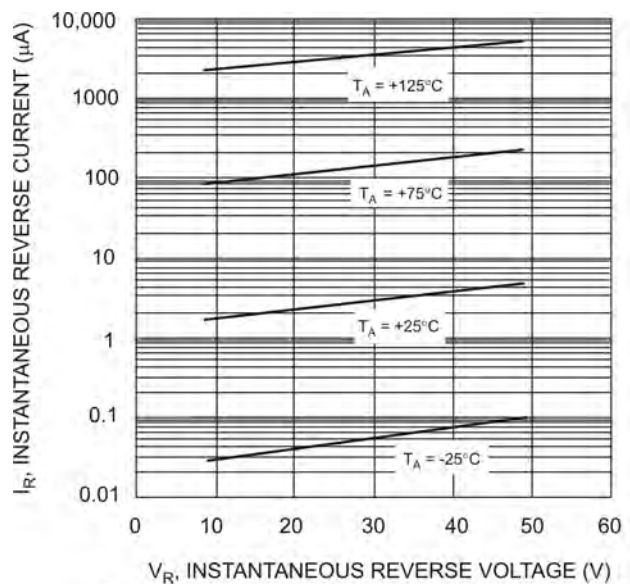
Fig. 6 Typical Reverse Characteristics, B320B thru B340B
