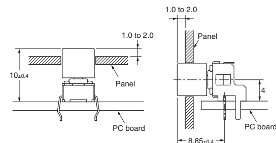
Reference Dimensions
