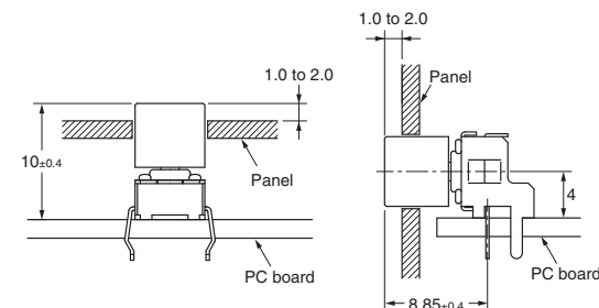
Reference Dimensions
