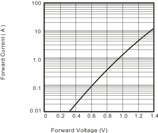
Fig.2 - Forward Characteristics
