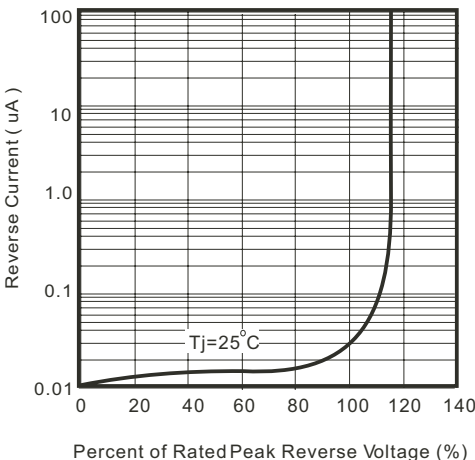
Fig. 1 - Reverse Characteristics
