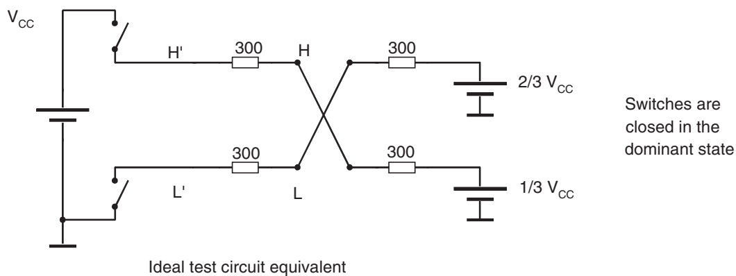
Figure 7-2. Test Circuit Equivalents
