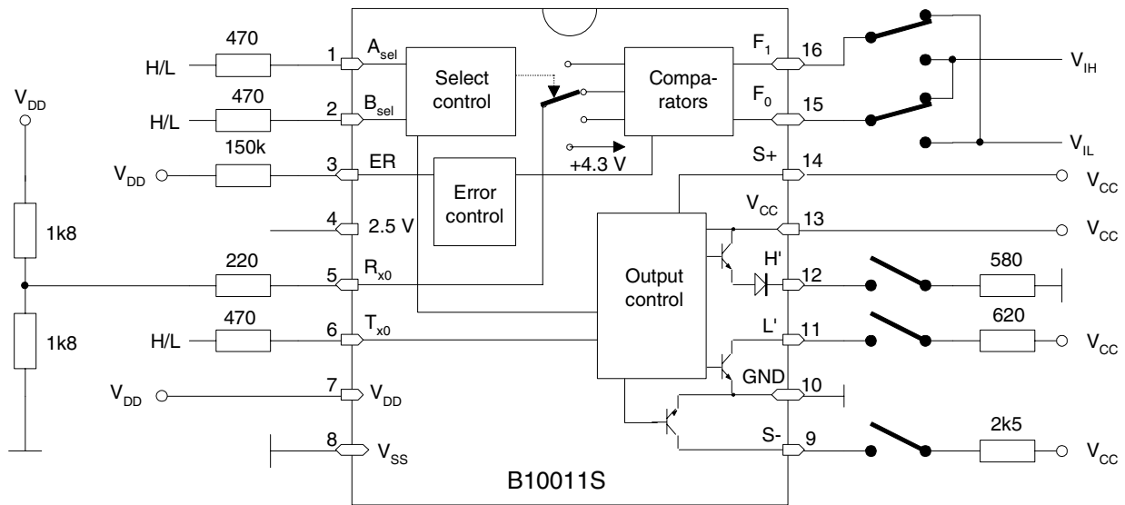
Figure 5. Application Circuit
