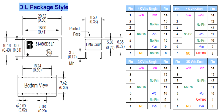
Dual Separate Output DIL Package Style
