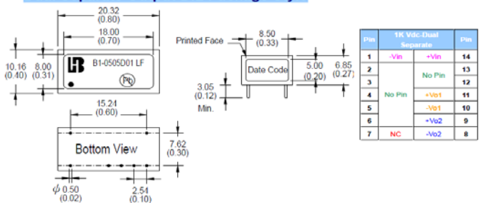
Dual Separate Output DIL Package Style
