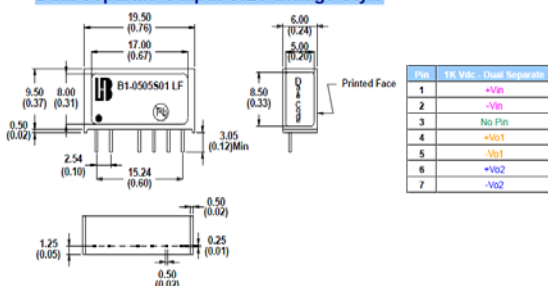
Dual Separate Output SIL Package Style
