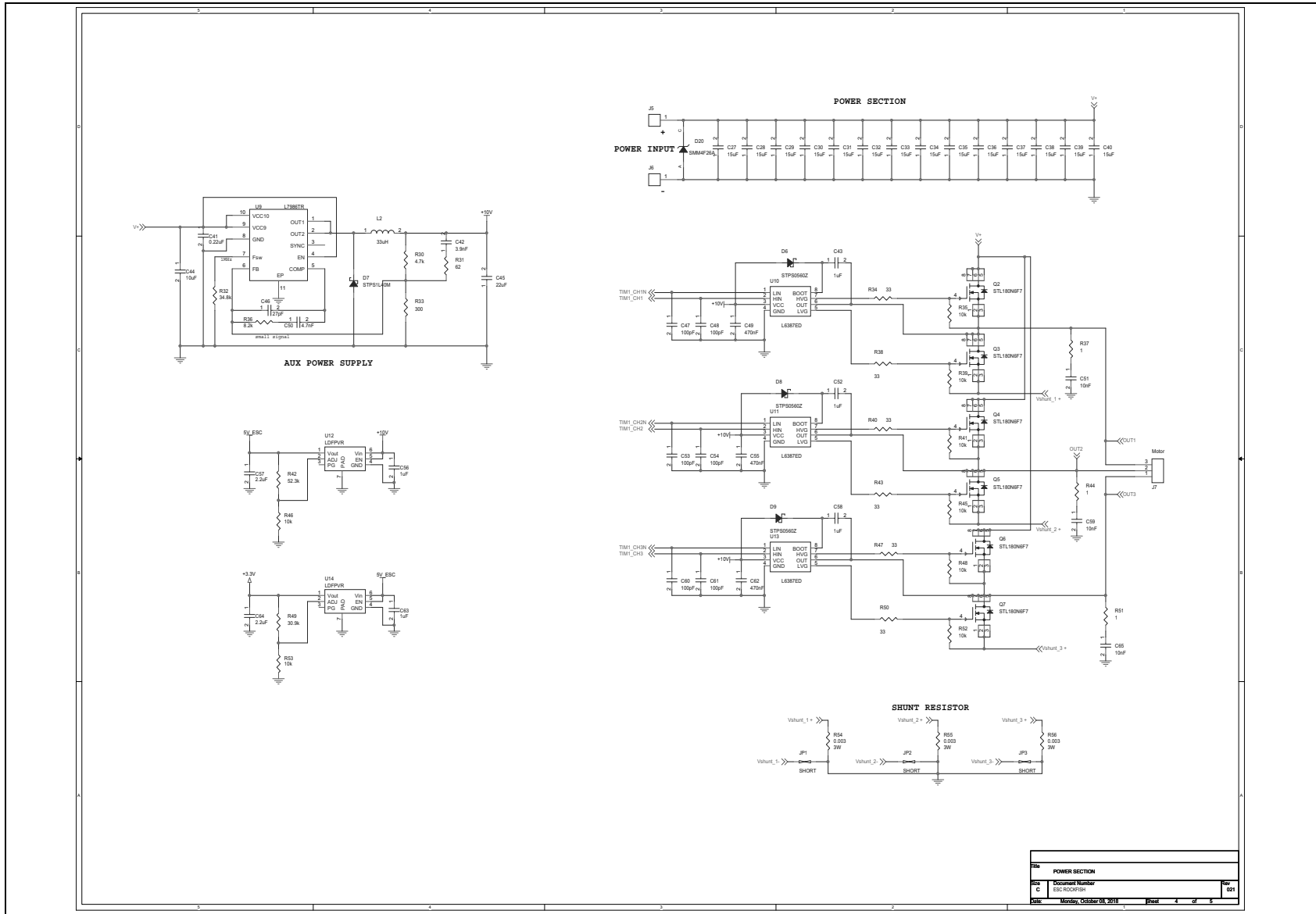
Figure 20. Power section
