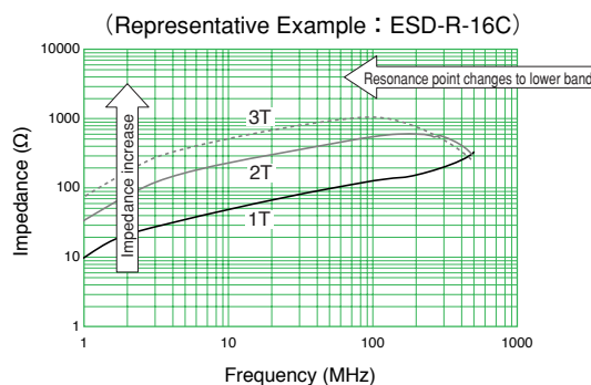
Fig.2 Relationship between impedance and turn counts
