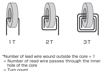
Fig.1 How to count turns
