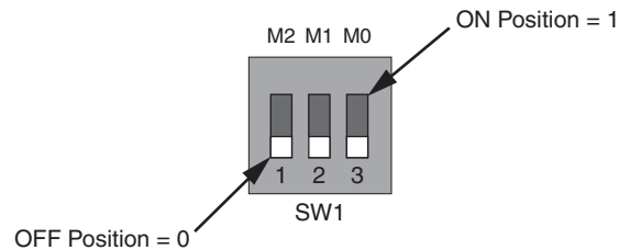
Figure 3: SW1 Switch Settings for JTAG Programming Mode
