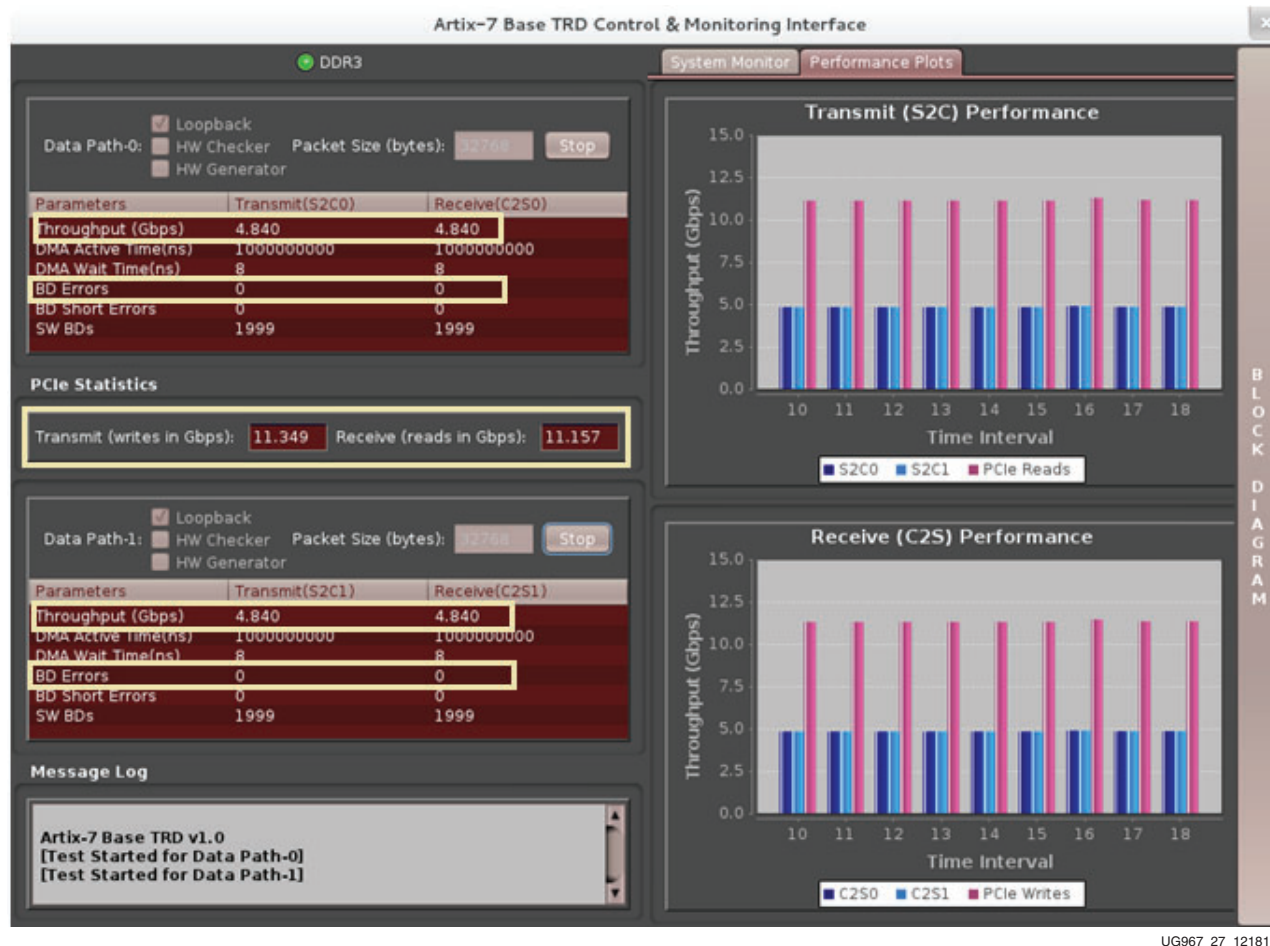
Figure 27: Verifying Error-free Operation and Performance Plots
