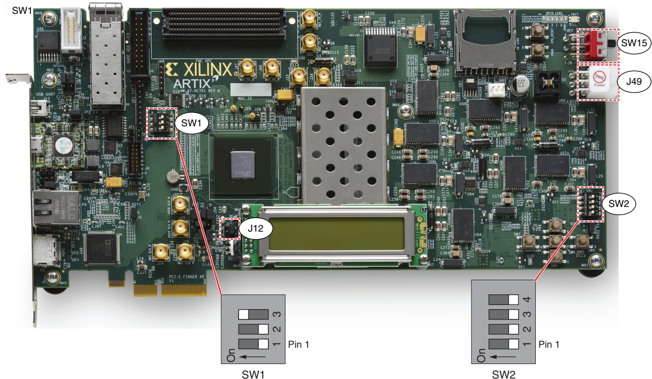
Figure 15: AC701 Board Switch and Jumper Locations
