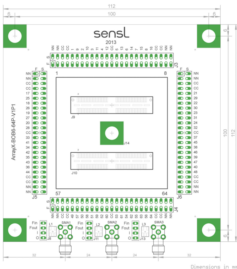
Figure 3. Layout of the ARRAYX-BOB6-64P. The dimensions of the board are 112 mm x 112 mm.
