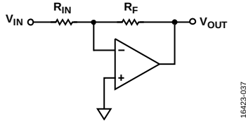
Figure 20. Inverting Amplifier
