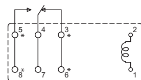
WIRING DIAGRAMS VIEWED TOWARDS TERMINALS
