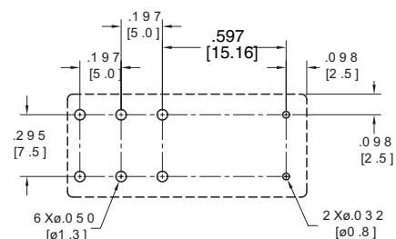
PC BOARD LAYOUT VIEWED TOWARDS TERMINALS
