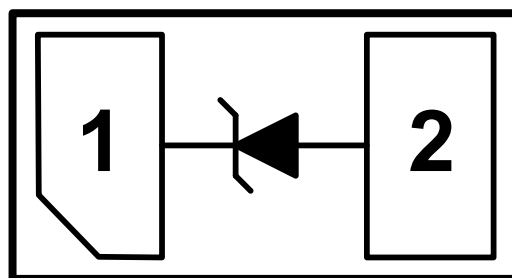
DFN1006P2X (Bottom View) (1.0mm x 0.6mm x 0.45mm)
