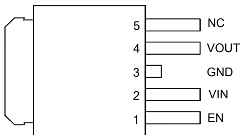
Figure 2. Pin Configuration of AZ39151 (Top View)
