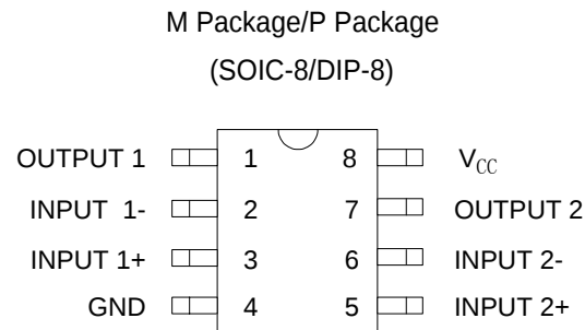
Figure 2. Pin Configuration of AZ358/358C (Top View)
