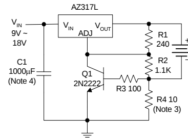
Figure 16. Current Limited 6V Charger Note 3: Sets peak current, I_{peak} = 0.6V/R4 Note 4: 1000μF is recommended to filter out any input transients.
