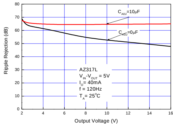
Figure 10. Ripple Rejection vs. Output Voltage
