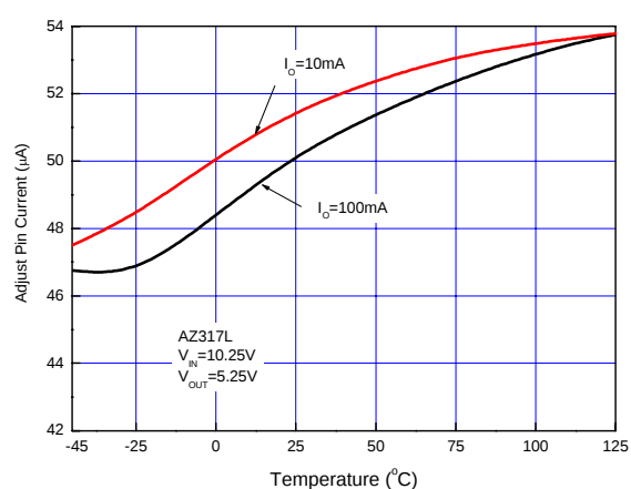
Figure 7. Adjustment Current vs. Temperature
