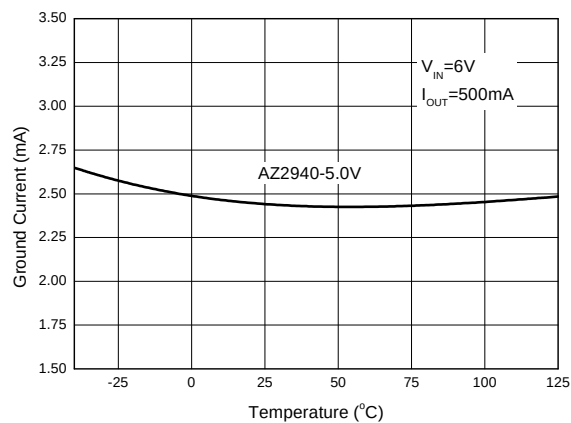
Figure 10. Ground Current vs. Temperature
