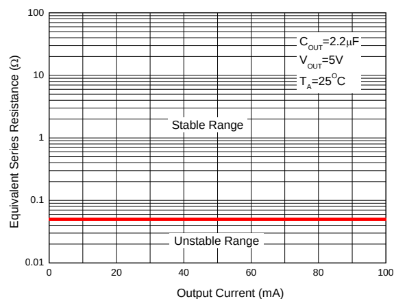
Figure 15. Output Capacitor ESR
