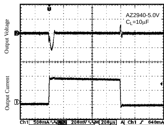
Figure 17. Load Transient
