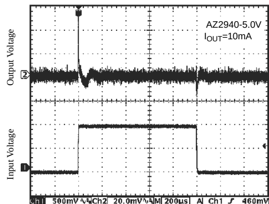
Figure 19. Line Transient
