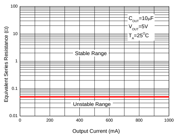
Figure 16. Output Capacitor ESR
