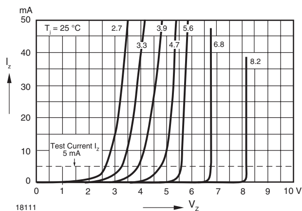
Figure 12. Breakdown Characteristics
