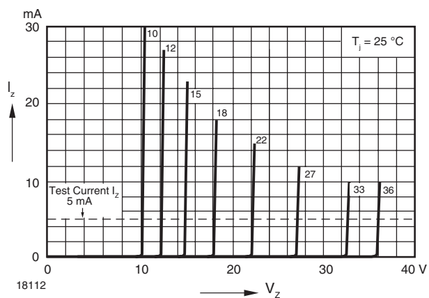
Figure 13. Breakdown Characteristics
