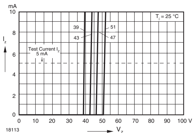
Figure 14. Breakdown Characteristics
