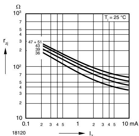
Figure 3. Dynamic Resistance vs. Zener Current
