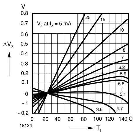
Figure 7. Change of Zener Voltage vs. Junction Temperature
