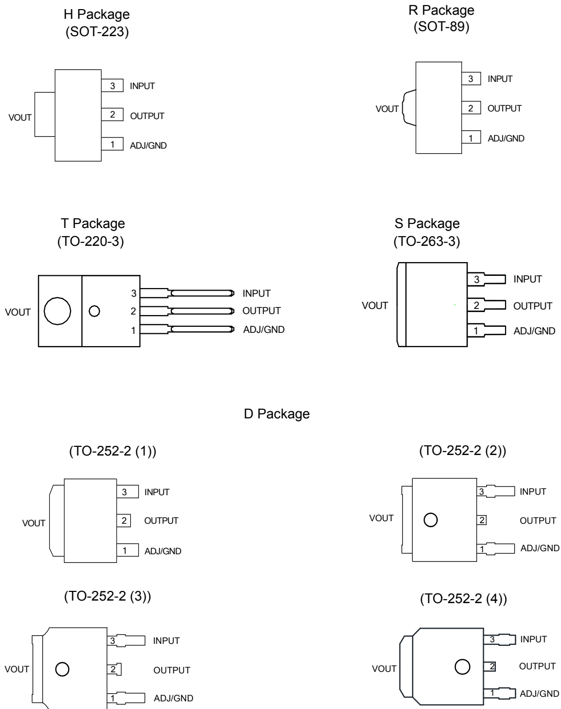
Figure 2. Pin Configuration of AZ1117
