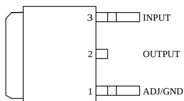
D Package (TO-252)
