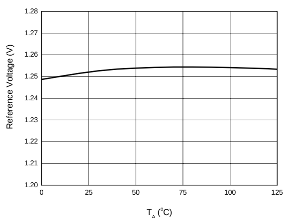
Figure10. Reference Voltage vs. Temperature
