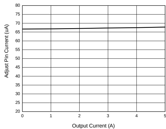
Figure 7. Adjust Pin Current vs. Output Current
