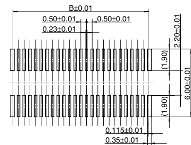
Recommended metal mask pattern Metal mask thickness: When 120 μm (Opening area ratio: 87%)
