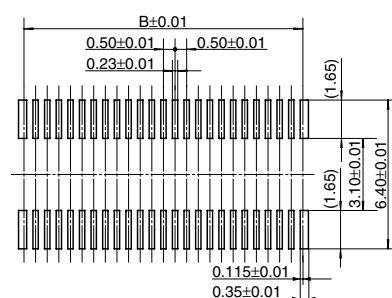
Recommended metal mask pattern Metal mask thickness: When 120 μm (Opening area ratio: 76%)
