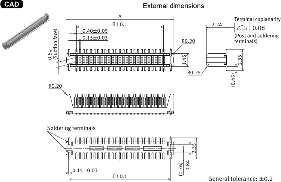
Dimension table
