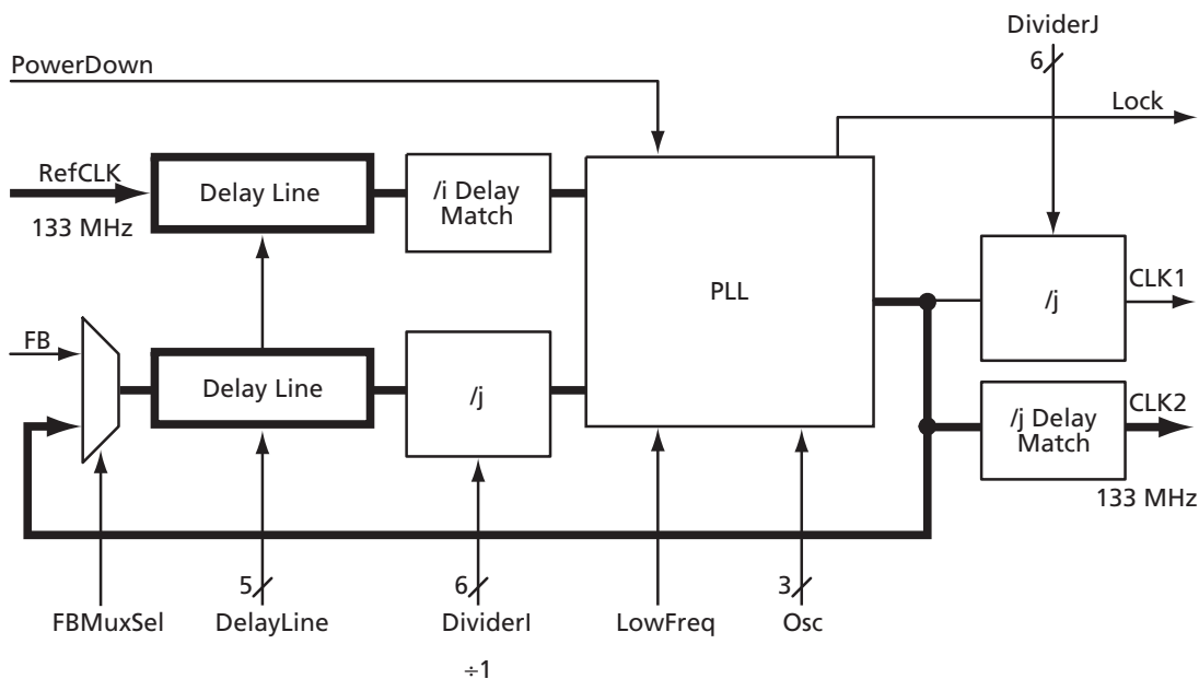
Figure 2-55 • Using the PLL Delaying the Reference Clock
