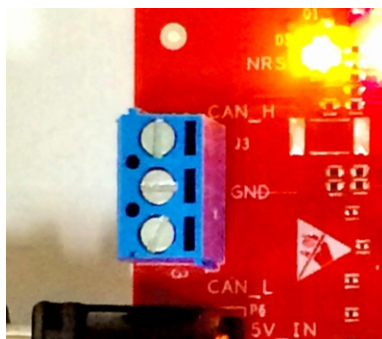
Figure 8. CAN Connector
