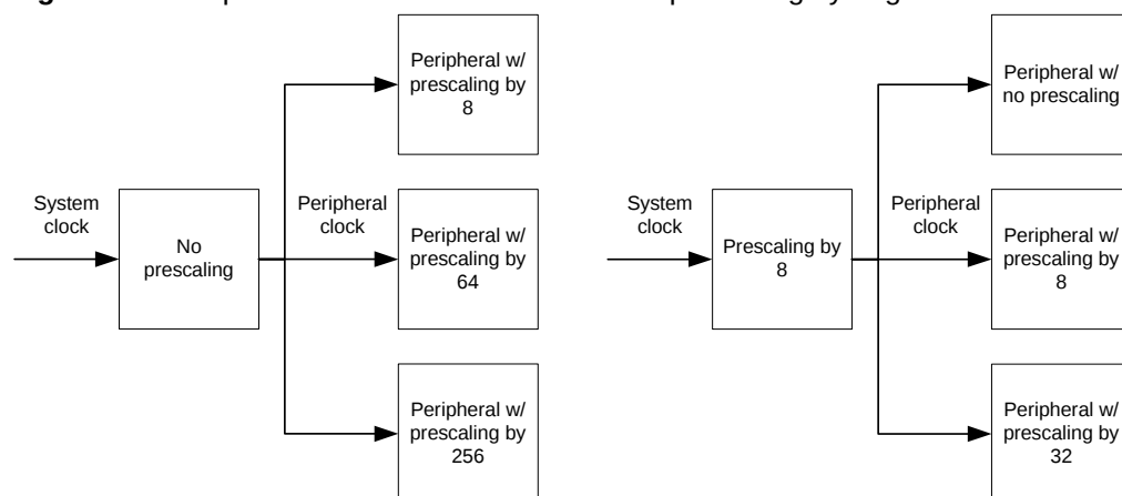
Figure 2-1: Peripherals without and with common prescaling by largest factor.
