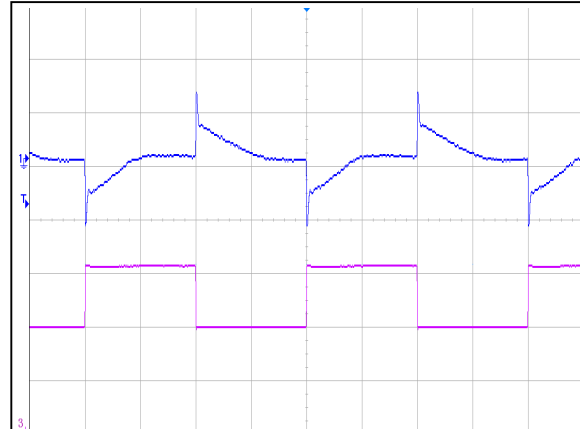
Figure 8: AVO250-48S28B Transient Response (2mS/div) 50%-75%~50% load change, 0.1A/uS slew rate, (50mV/div) Ch 1: Vo Ch 3: Io (2A/div)
