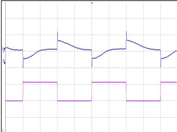
Figure 7: AVO250-48S28B Transient Response (2mS/div) 25%-50%~25% load change, 0.1A/uS slew rate, (50mV/div) Ch 1: Vo Ch 3: Io (2A/div)
