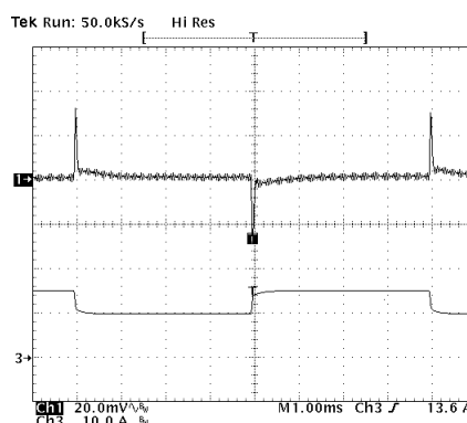
Typical Transient Response to Step Load Change from 50%-75%I max , AV45C-048L-018F20HAN
