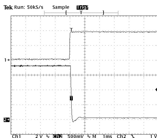
Typical Shut-down Transient with CNT AV45C-048L-018F20HAN
