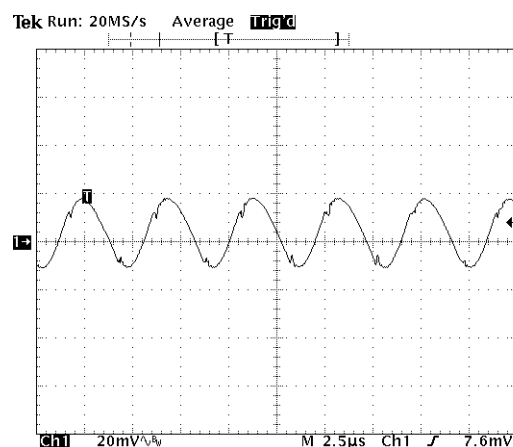
Typical Output Ripple Voltage AV45C-048L-018F20HAN
