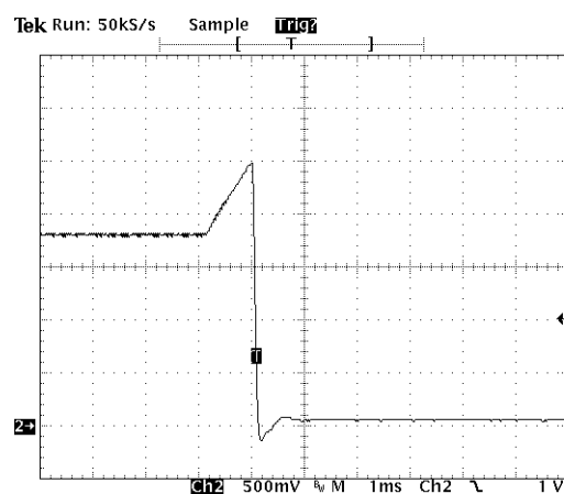
Overvoltage Protection AV45C-048L-018F20HAN
