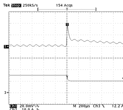
Typical Transient Response to Step Load Change from 50%-75%-50%I max , AV45C-048L-018F20HAN
