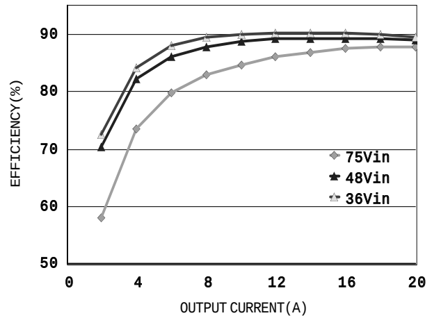
Typical Efficiency AV45C-048L-033F20HAN
