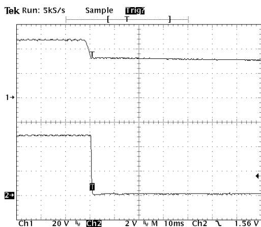
Typical Shut-down from Power Off AV45C-048L-050F20HAN
