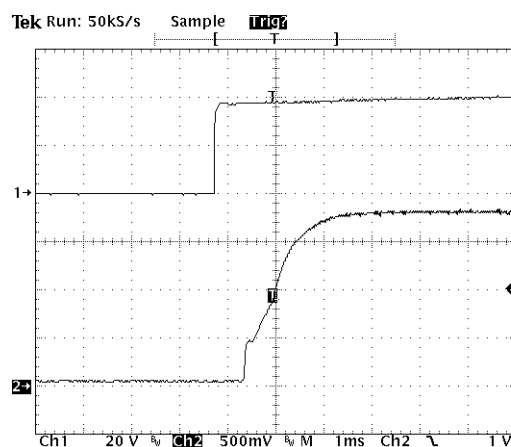
Typical Start-Up from Power On AV45C-048L-018F20HAN
