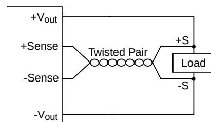
Fig.9 Sense Connections
