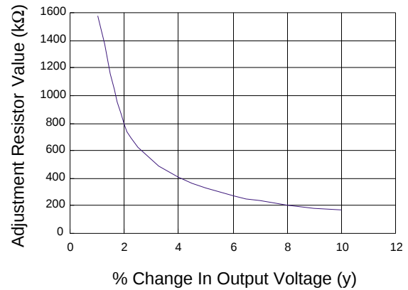
Fig.12 Resistor Selection for 5Vout Trimming Up
