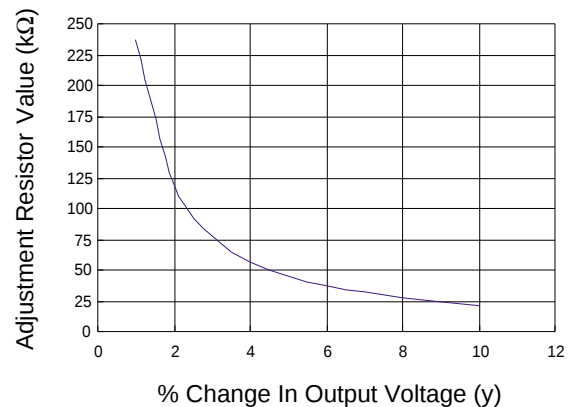
Fig.13 Resistor Selection for 1.8Vout Trimming Up
