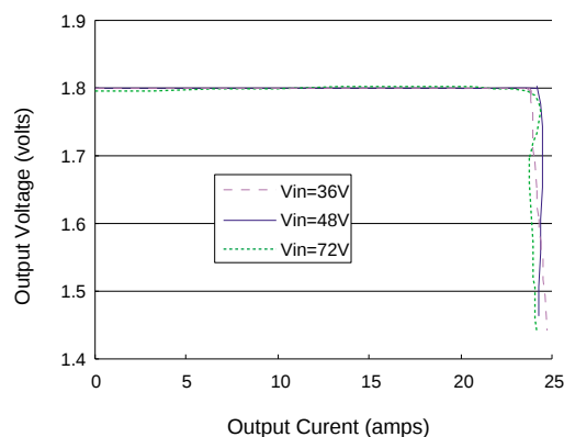
Typical Output Overcurrent Characteristics AV45C-048L-018F20HAN
