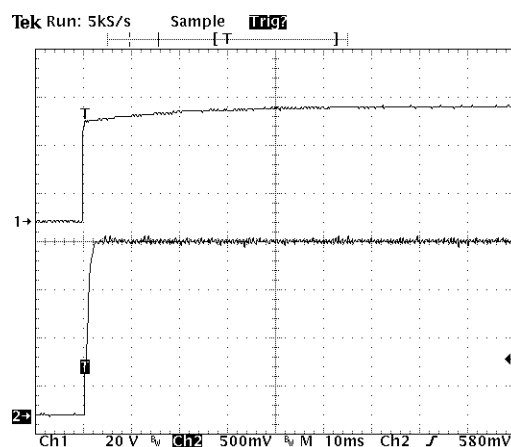
Typical Start-Up Transient with CNT AV45C-048L-018F20HAN
