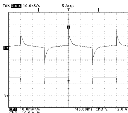
Typical Transient Response to Step Load Change from 50%-75%I max , AV45C-048L-050F20HAN
