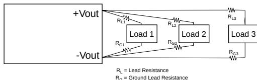
Fig.20 Radial Power Distribution
