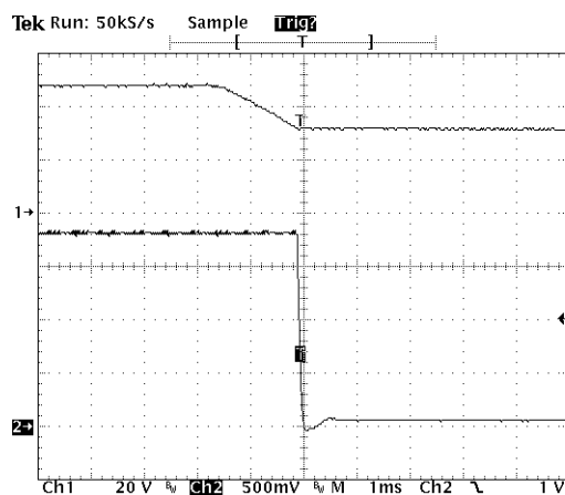
Typical Shut-down from Power Off AV45C-048L-018F20HAN
