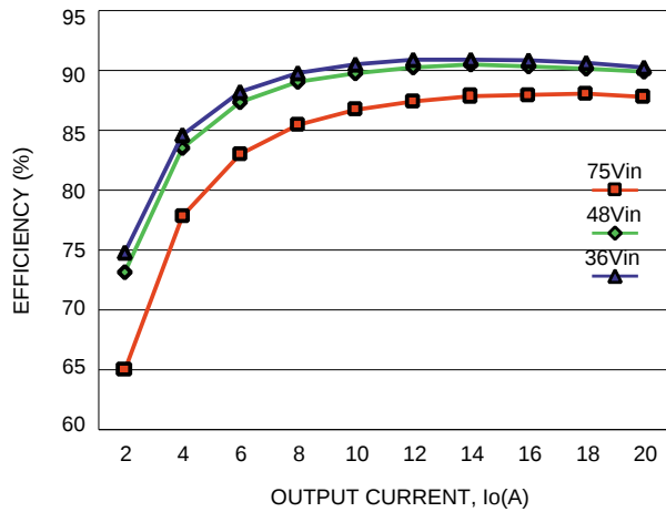
Typical Efficiency AV45C-048L-050F20HAN
