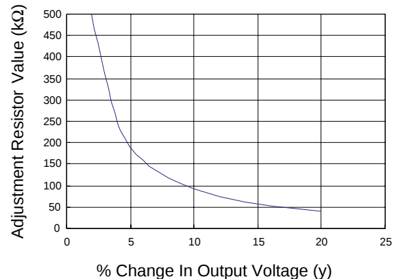
Fig.14 Resistor Selection for Trimming Down Output
