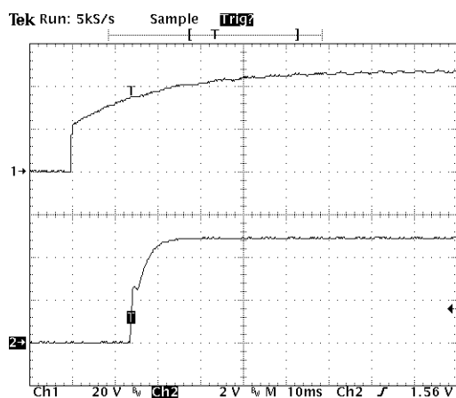
Typical Start-Up from Power On AV45C-048L-050F20HAN
