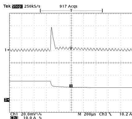
Typical Transient Response to Step Load Change from 75%-50%I max , AV45C-048L-018F20HAN
