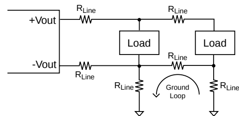
Fig.17 Ground Loops
