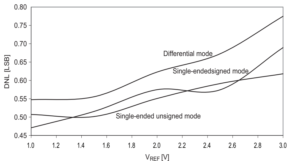
Figure 37-204. DNL error vs. external V_{REF} . T = 25^{\circ}\text{C} , V_{CC} = 3.6\text{V} , external reference.
