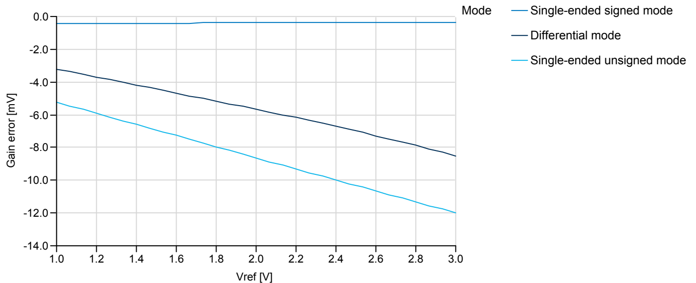
Figure 37-42. ADC Gain Error vs. V_{REF}
