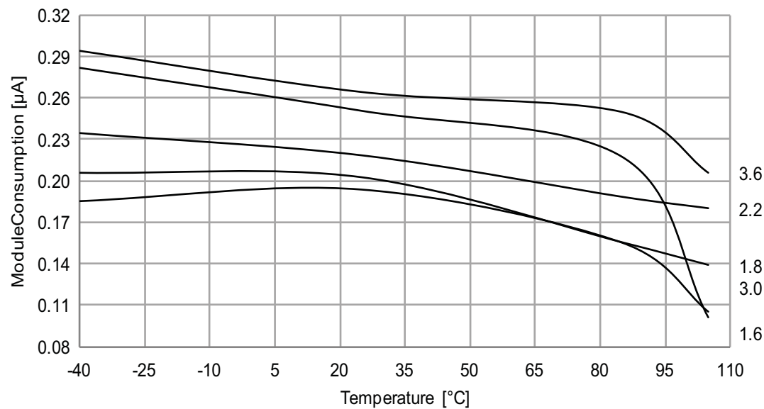
Figure 37-88. P_{SAVE} vs. Temperature RTC, WDT, BOD sampled.
