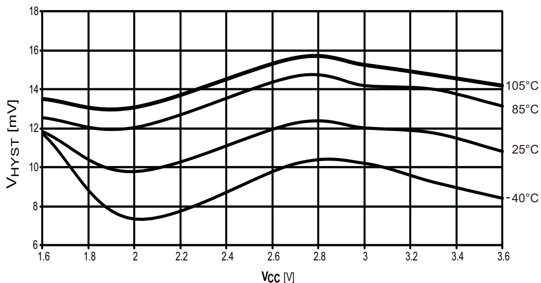
Figure 37-44. Analog Comparator Hysteresis vs. V_{CC}
