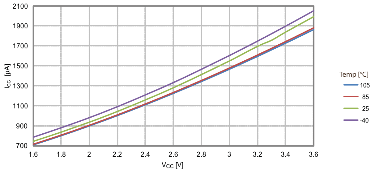
Figure 37-11. Idle Mode Supply Current vs. V_{CC} f_{SYS} = 32\text{MHz} internal oscillator prescaled to 8MHz.
