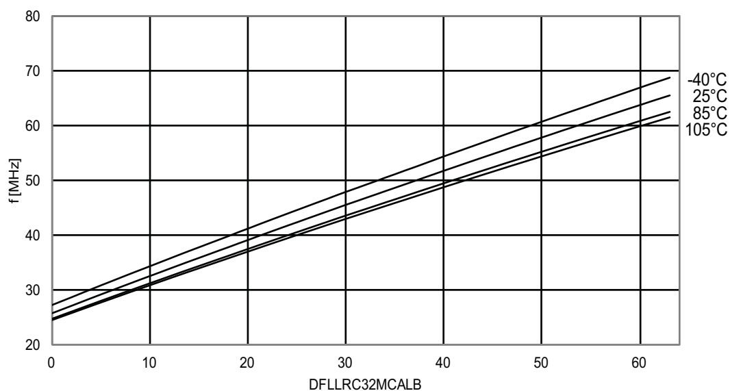
Figure 37-75. 32MHz Internal Oscillator Frequency vs. CALB Calibration Value
