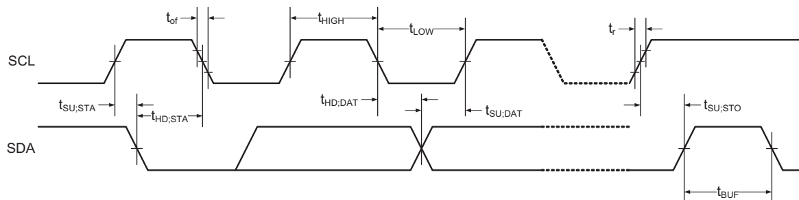
Figure 36-7. Two-wire Interface Bus Timing
