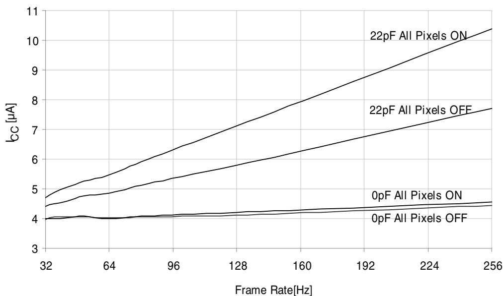
Figure 37-82. I_{CC} vs. Frame Rate
