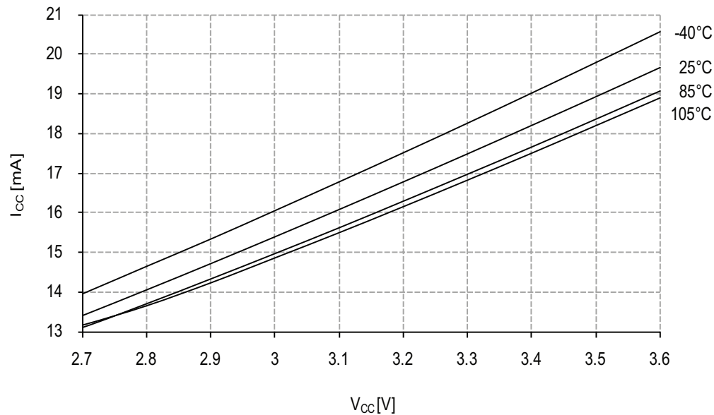
Figure 38-89. Active mode supply current vs. V_{CC} .
