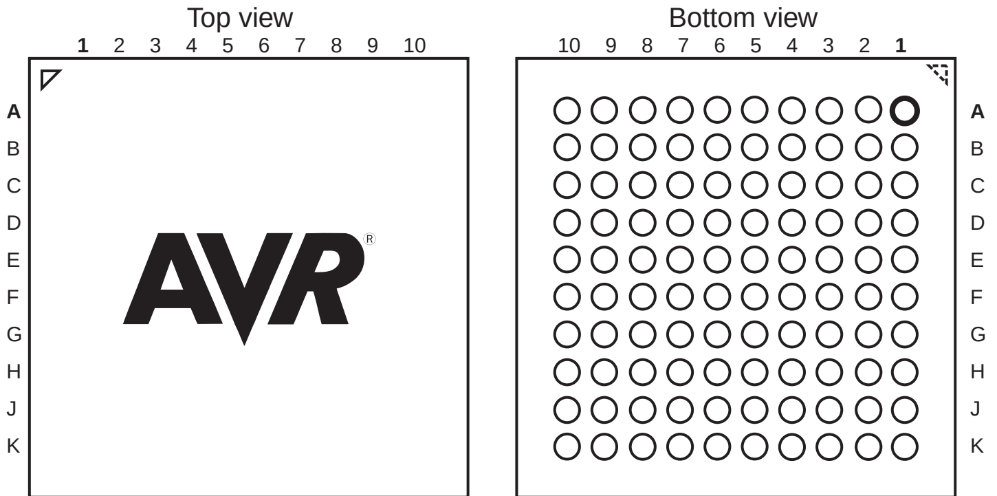
Figure 2-2. BGA-pinout.
