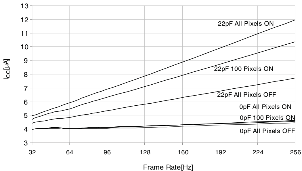
Figure 37-77. I_{CC} vs. Frame Rate
