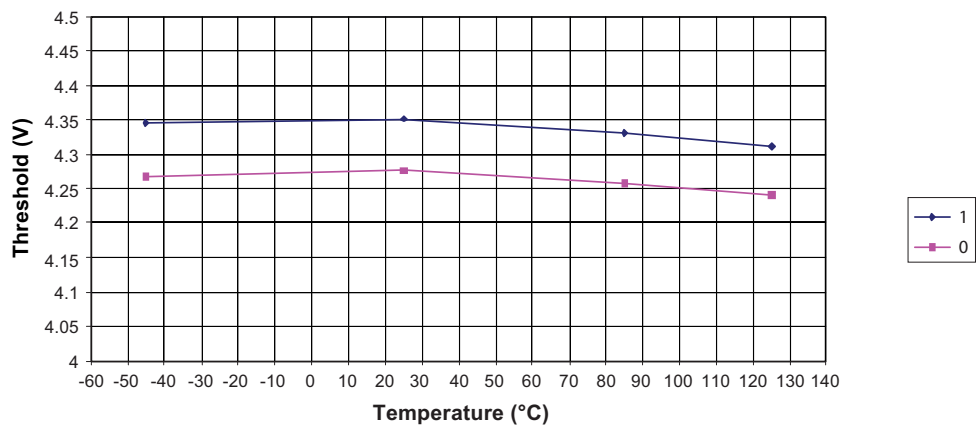
Figure 22-15. BOD Threshold versus Temperature (BOD Level is 4.3V)
