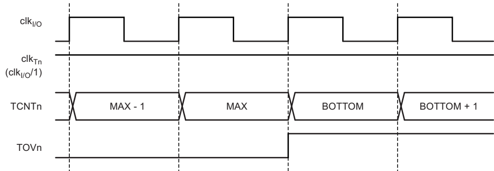
Figure 11-5. Timer/Counter Timing Diagram, no Prescaling
