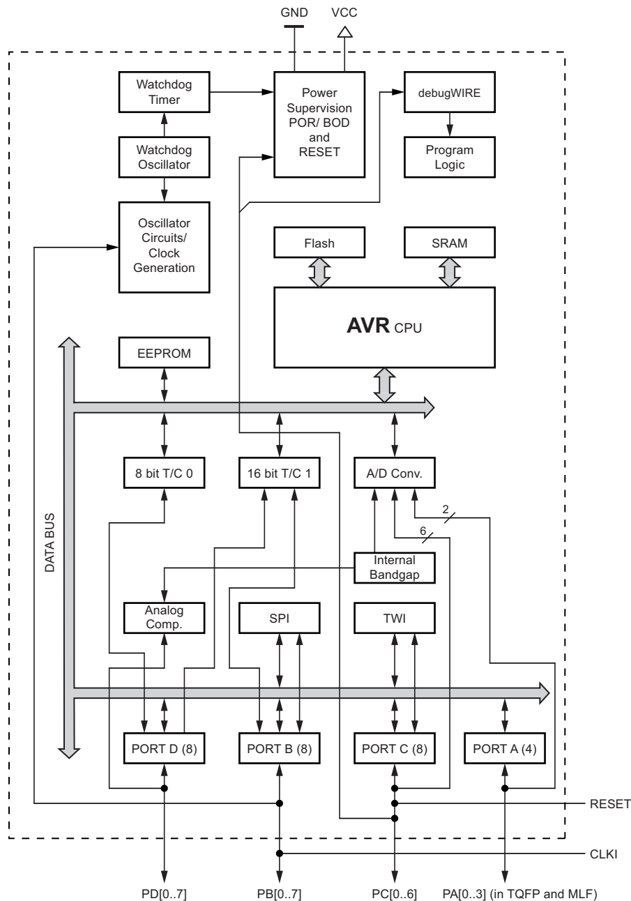
Figure 2-1. Block Diagram
